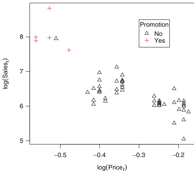
Figure 9.1 A scatter plot of log(Sales t ) against log(Price t )
