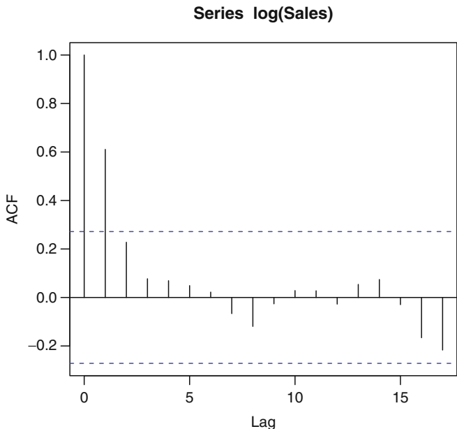
Figure 9.4 Autocorrelation function for \log(\text{Sales})
