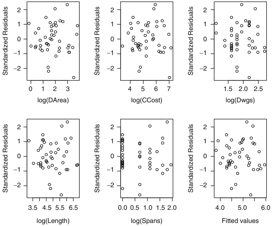
Figure 6.41 Plots of the standardized residuals from model (6.28)
