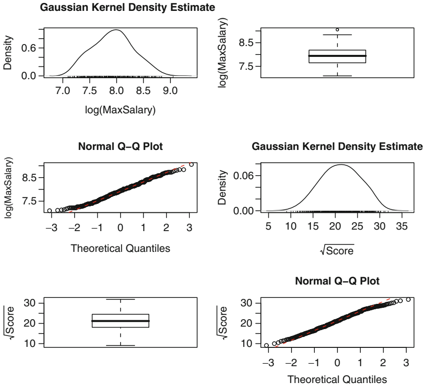
Figure 3.35 Plots of the transformed data
