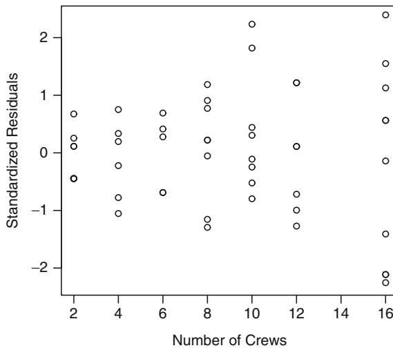
Figure 3.16 Plot of standardized residuals against x , number of cleaning crews
