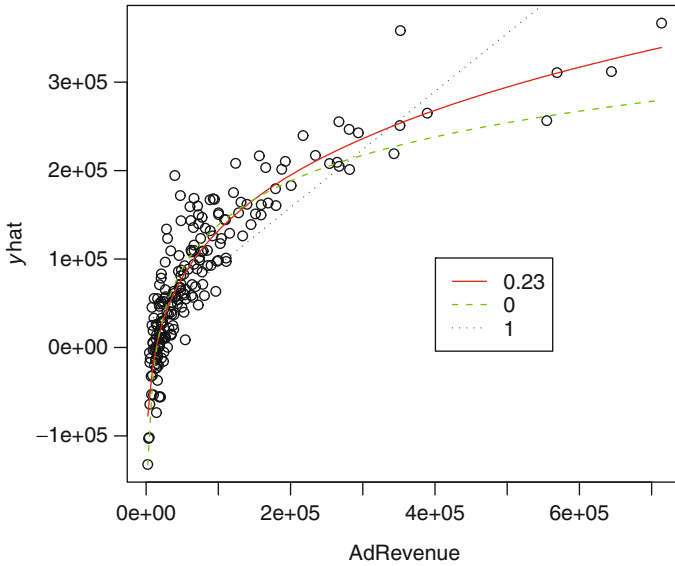
Figure 6.22 Inverse response plot
