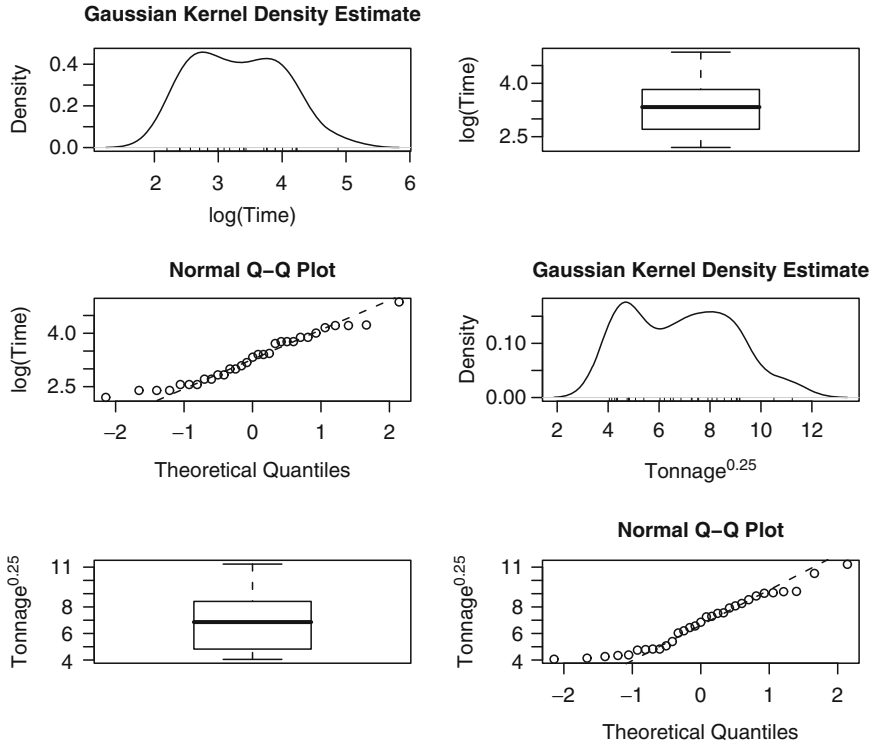
Figure 3.45 Density estimates, box plots and Q-Q plots of log(Time) and Tonnage 0.25
