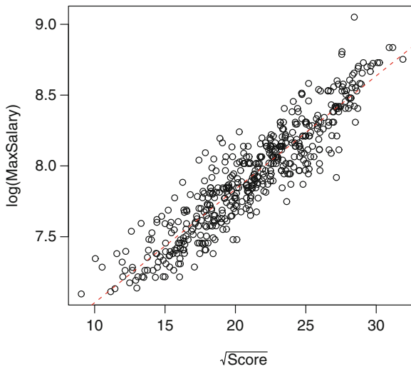
Figure 3.34 Plot of \log(\text{MaxSalary}) and \sqrt{\text{Score}} with the least squares line added
