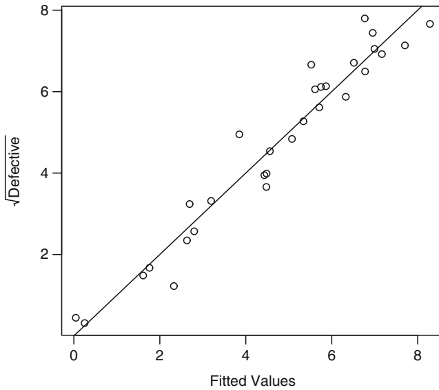
Figure 6.18 A plot of Y^{0.5} against fitted values with a straight line added
