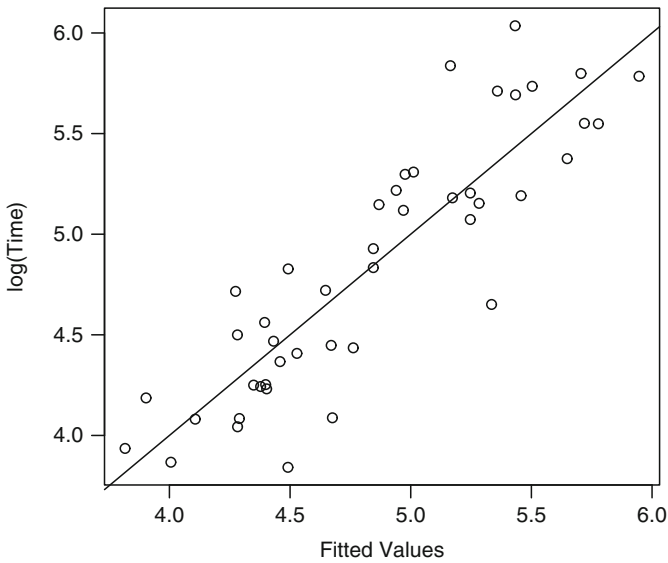
Figure 6.42 A plot of log(Time) against fitted values with a straight line added
