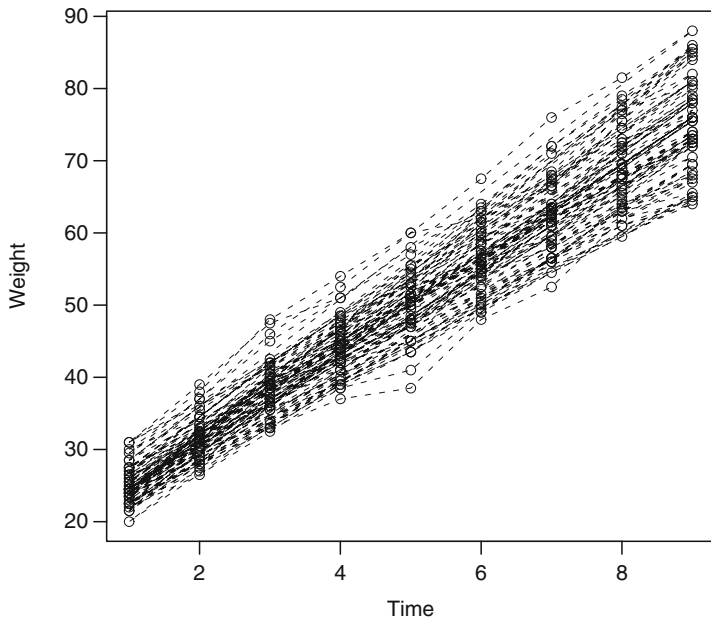
Figure 10.13 Plot of pig weights over time
