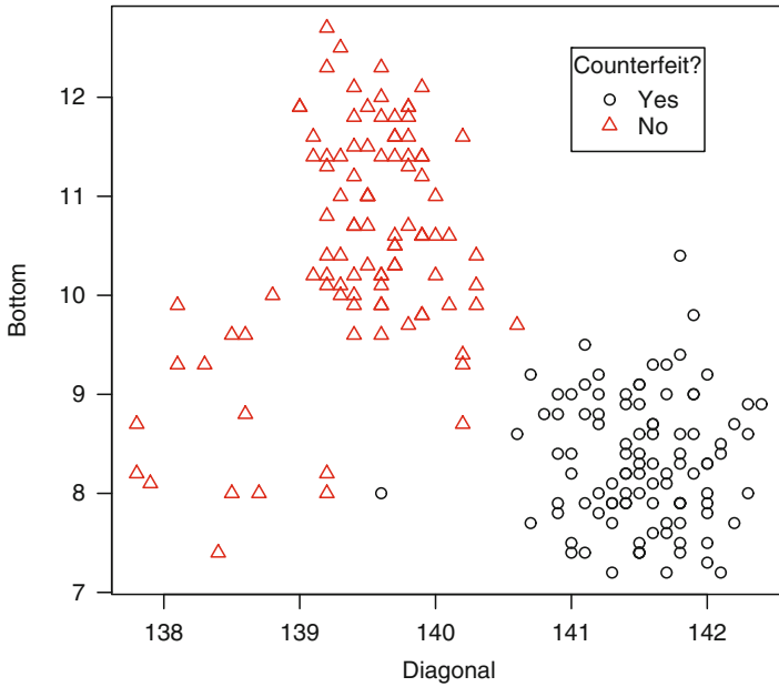
Figure 8.20 A plot of two of the predictors of counterfeit Swiss Bank notes
