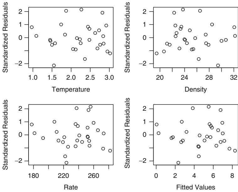
Figure 6.17 Plots of the standardized residuals from model (6.15)
