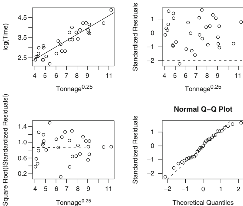
Figure 3.44 Output from model (3.9)
