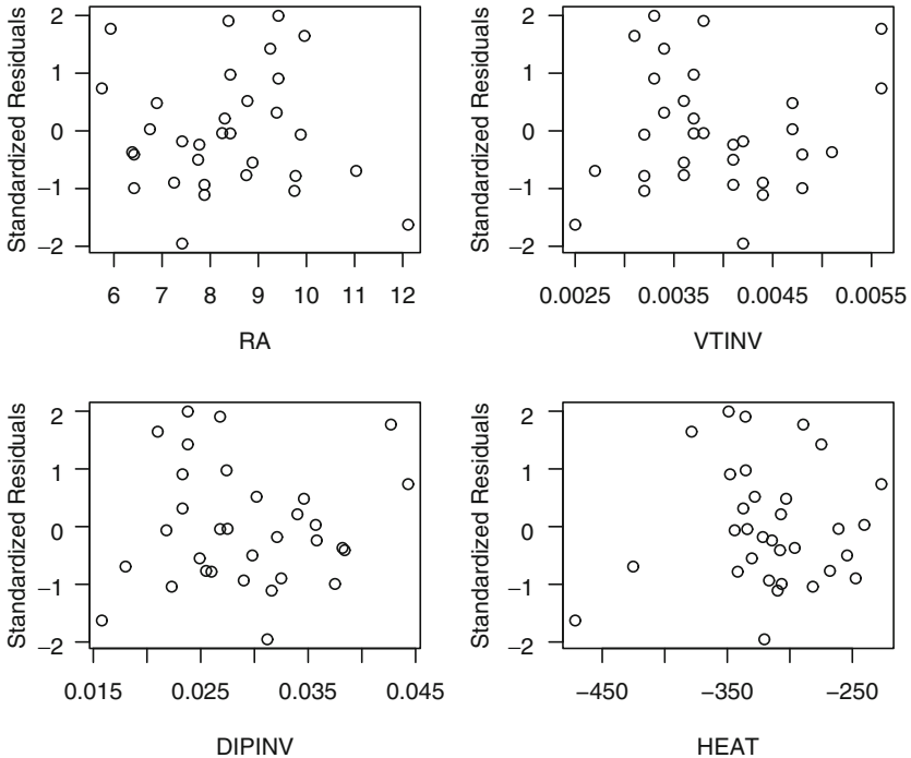
Figure 6.60 Plots of standardized residuals from model (6.38)
