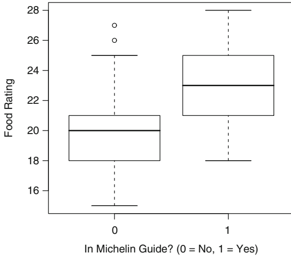
Figure 8.5 Box plots of Food Ratings
