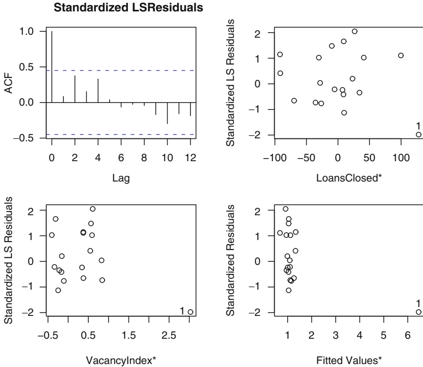
Figure 9.15 Plots of standardized LS residuals from model (9.6)
