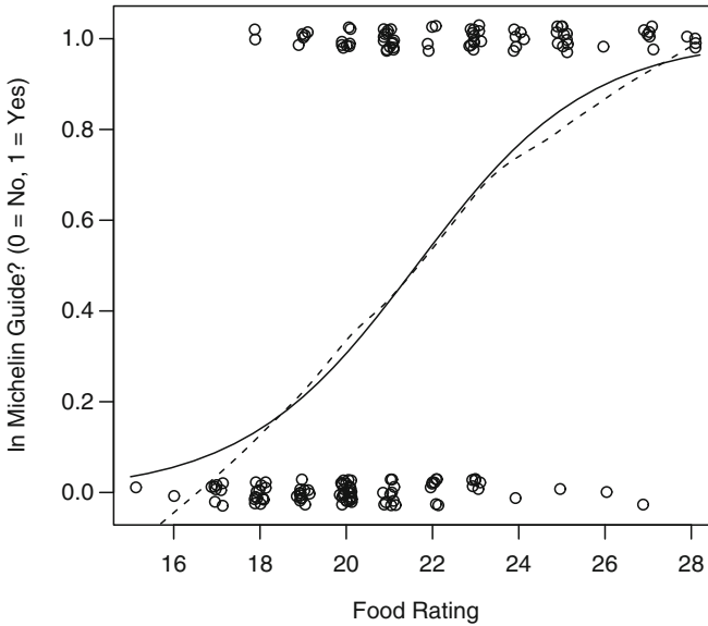
Figure 8.7 Plot of y_i versus food rating with the logistic and loess fits added
