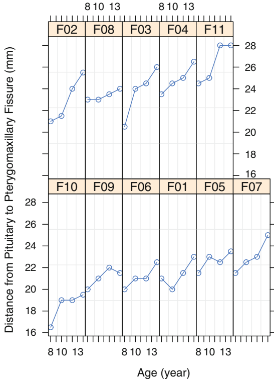
Figure 10.1 Plot of Distance against Age for each female
