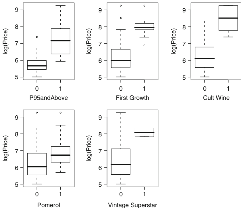
Figure 1.10 Box plots of log(Price) against each of the dummy variables
