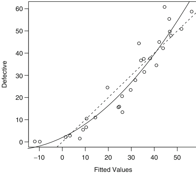
Figure 6.13 Plot of Y against fitted values with a straight line and a quadratic curve
