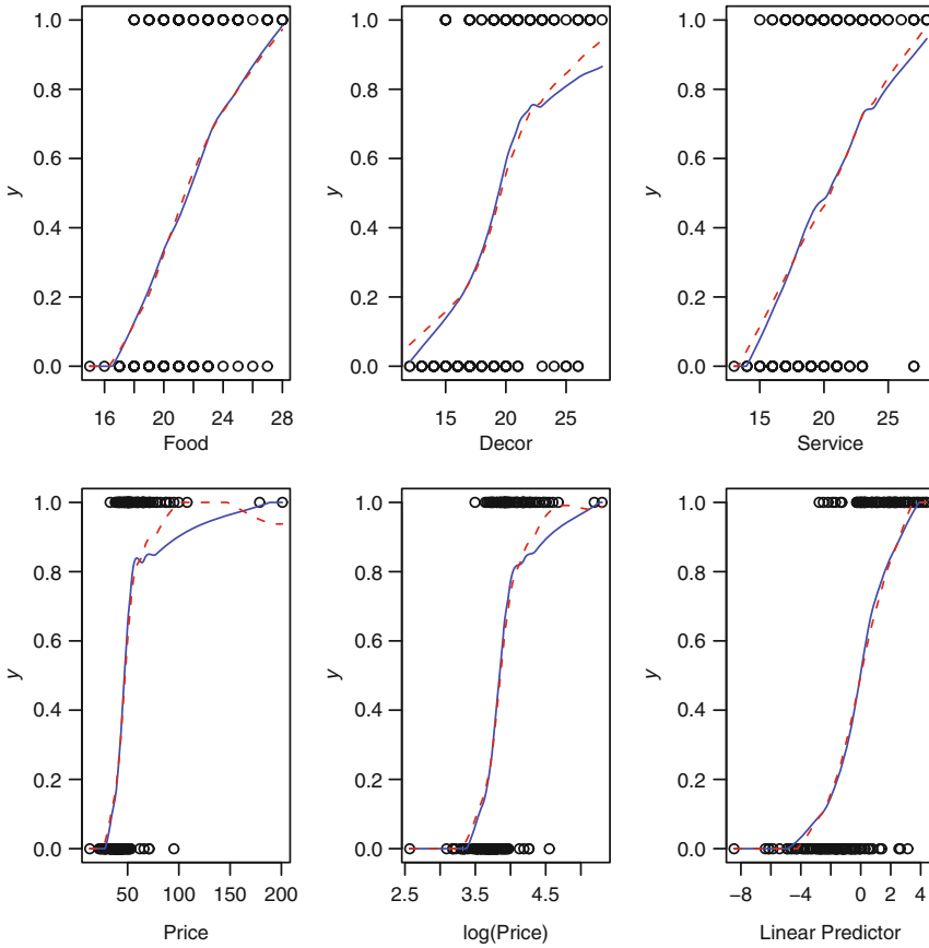
Figure 8.12 Marginal model plots for model (8.4)
