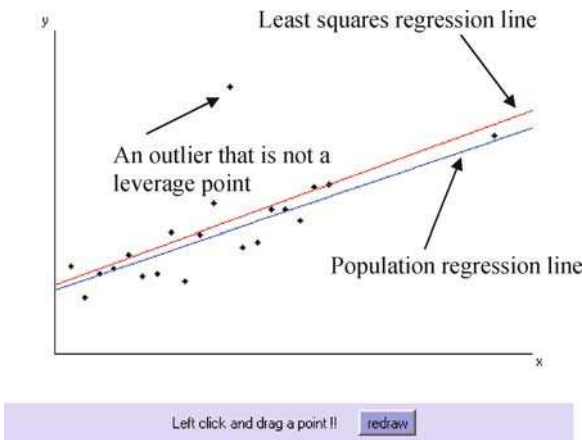
Figure 3.6 A plot of Y against x showing an outlier that is not a leverage point
