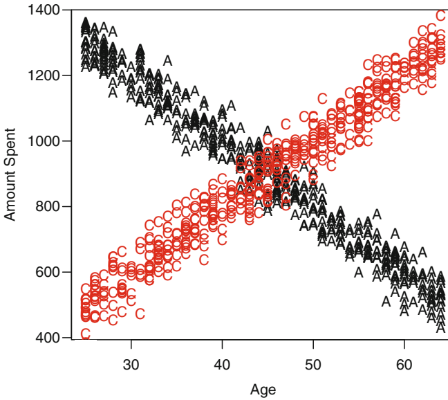
Figure 5.7 A scatter plot of Amount Spent versus Age for segments A and C
