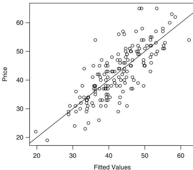
Figure 6.3 A plot of Price against fitted values
