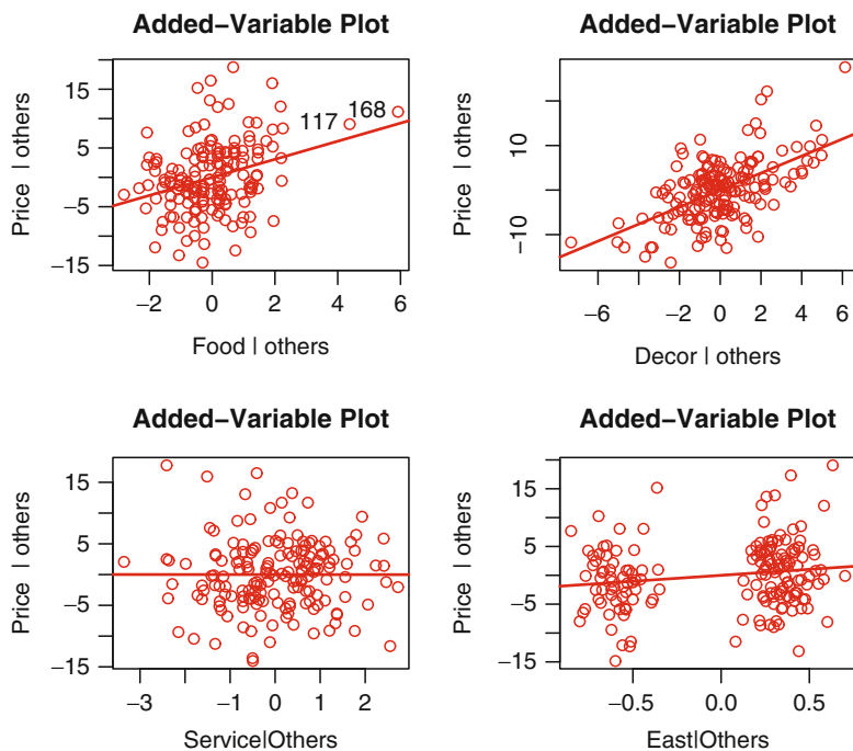
Figure 6.10 Added-variable plots for the New York City restaurant data
