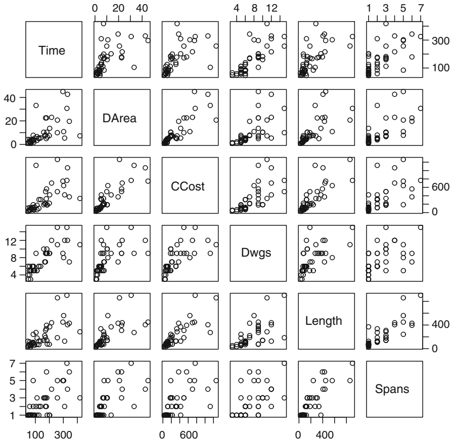
Figure 6.39 Scatter plot matrix of the response variable and each of the predictors
