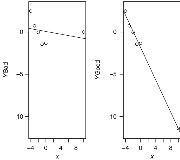
Figure 3.7 Plots of YGood and YBad against x with the fitted regression lines
